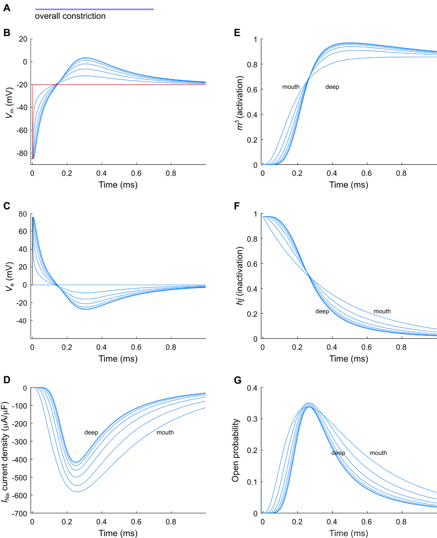
Supplemental figure 4. Modeling sodium current in an 5.4- \mu\text{m} -long overall constricted murine T-tubule. (A), Schematic representation of the morphology of the tubule (compare to Figure 6 where L = 9 \mu\text{m} ). Membrane potentials (B), extracellular potentials (C), and simulated sodium current density upon a voltage-clamp step of the tubule mouth from -85 to -20 mV (D) are given. Panels E-G show the biophysical properties of the sodium current, including activation gates ( m^3 , E), inactivation gates ( hj , F), and open probability (defined as m^3hj , G). Data are shown for every tenth node.
